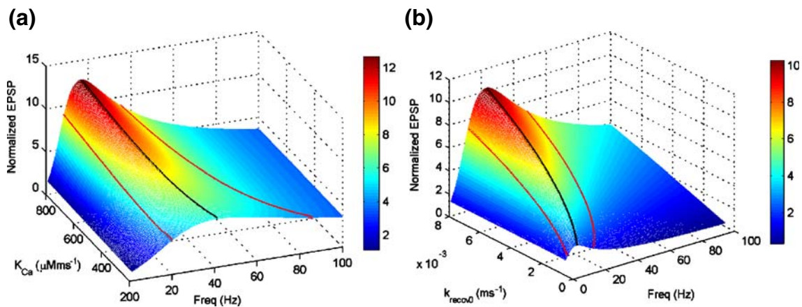
Fig. 7 Frequency response surfaces constructed by changing physiological parameters based on Eq. (11). The center line indicates the resonance frequency and the lines on the both sides label the half-
